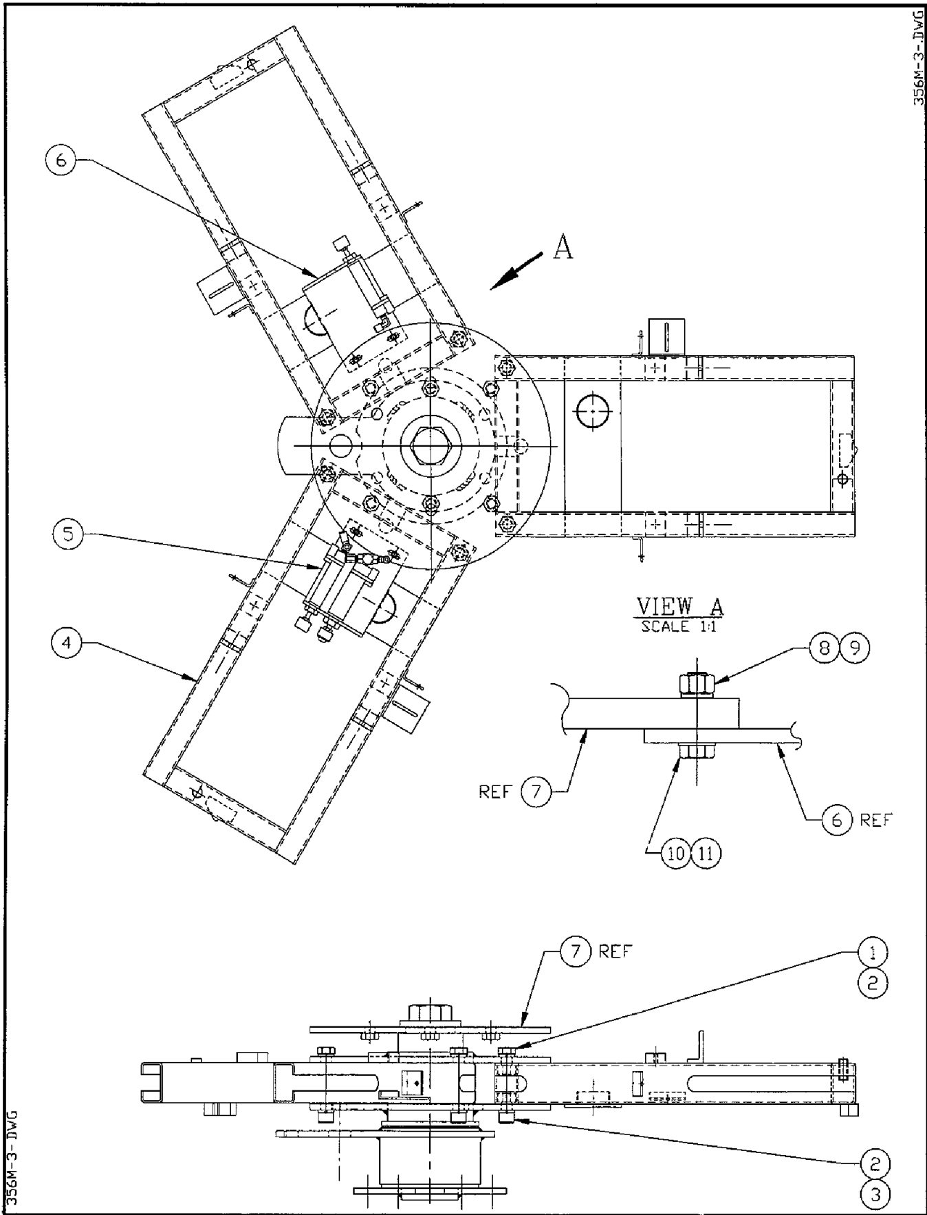
Figure 6-19. Buck Support Assembly
