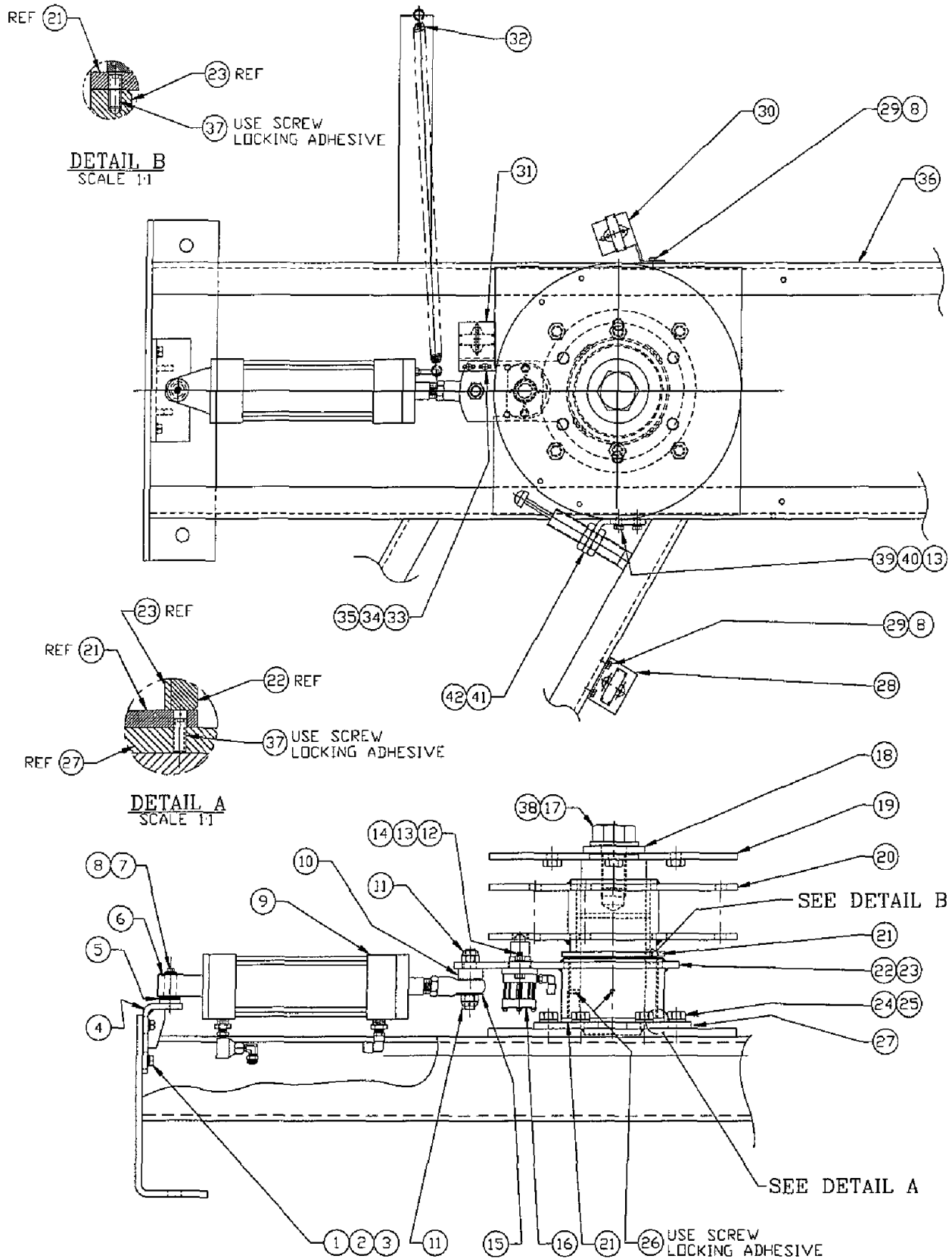
Figure 6-22. Indexing Assembly
