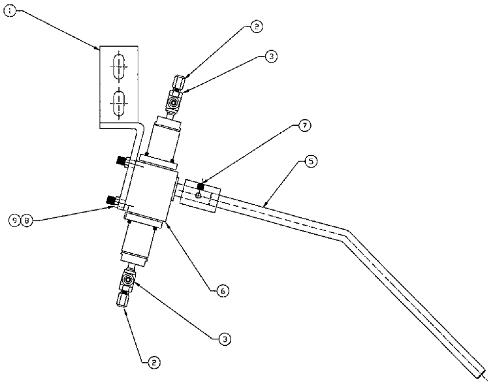
Figure 6-47. Mendline Assembly Option, Fits Left Hand Unloading
