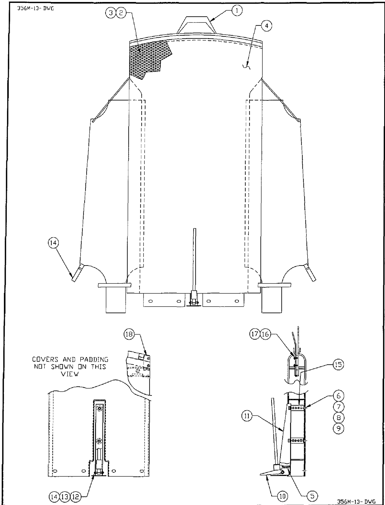
Figure 6-28. Buck Assembly
