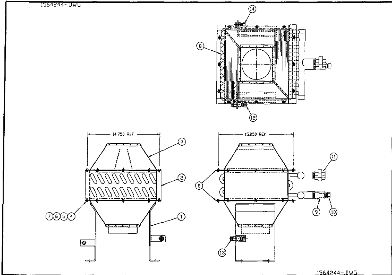
Figure 6-38. Steam Coil
