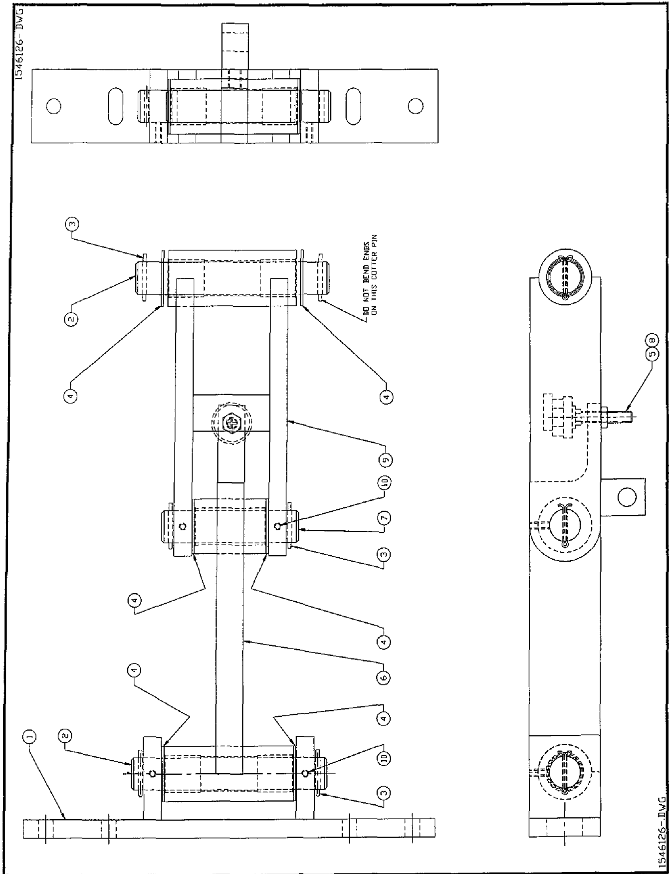
Figure 6-8. Linkage Assembly
