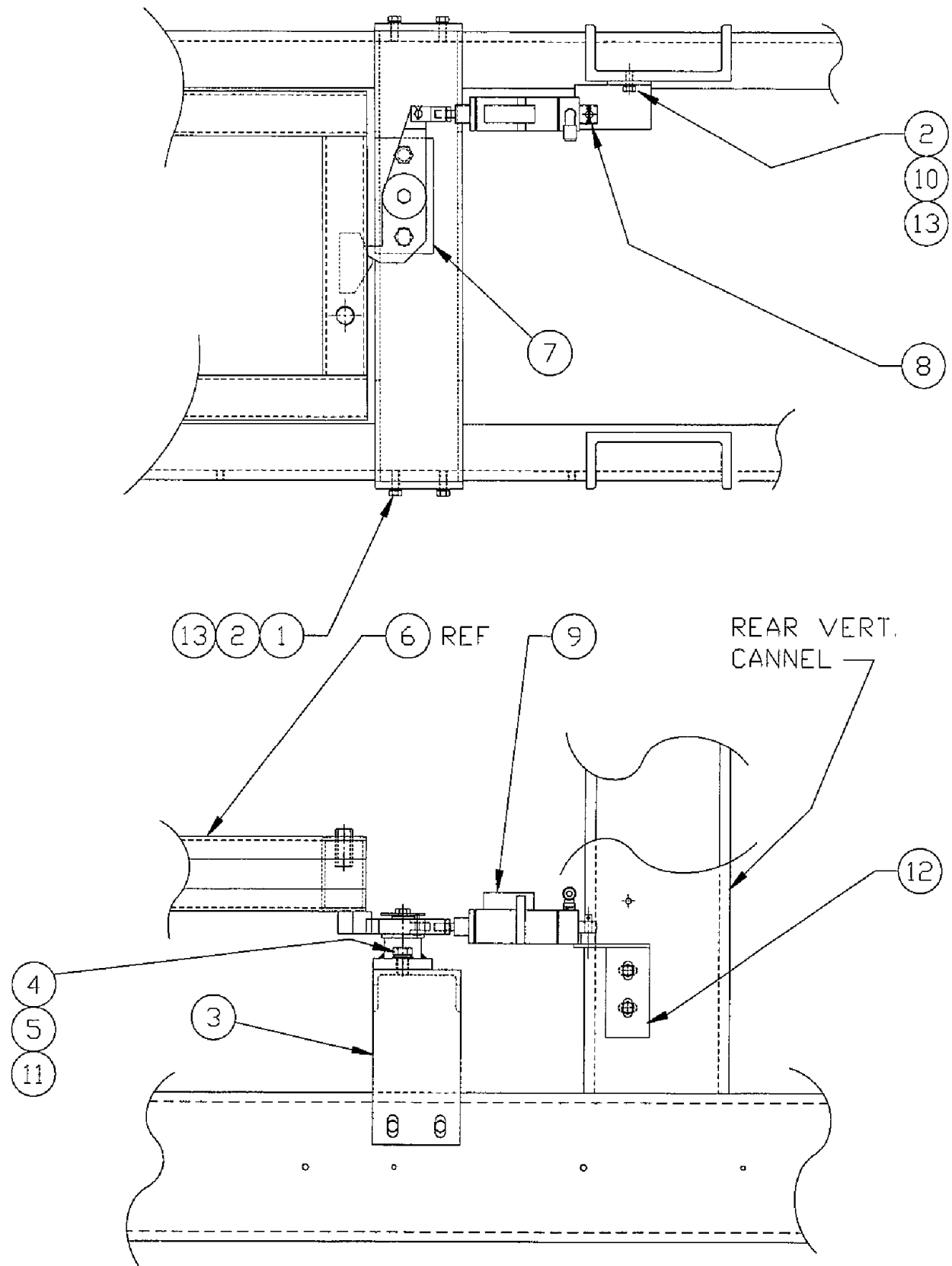
Figure 6-25. Buck Locking Assembly
