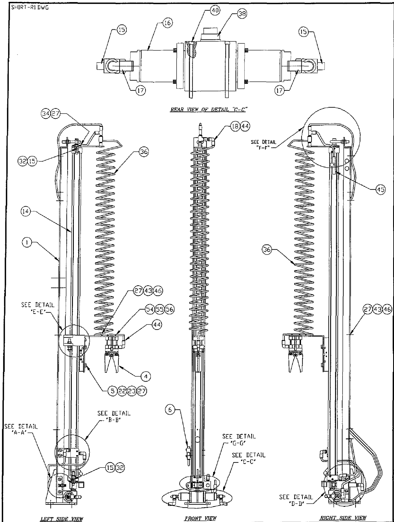
Figure 6-44. Shirt Take-Away, Right Hand Assembly (Sheet 1 of 2)
