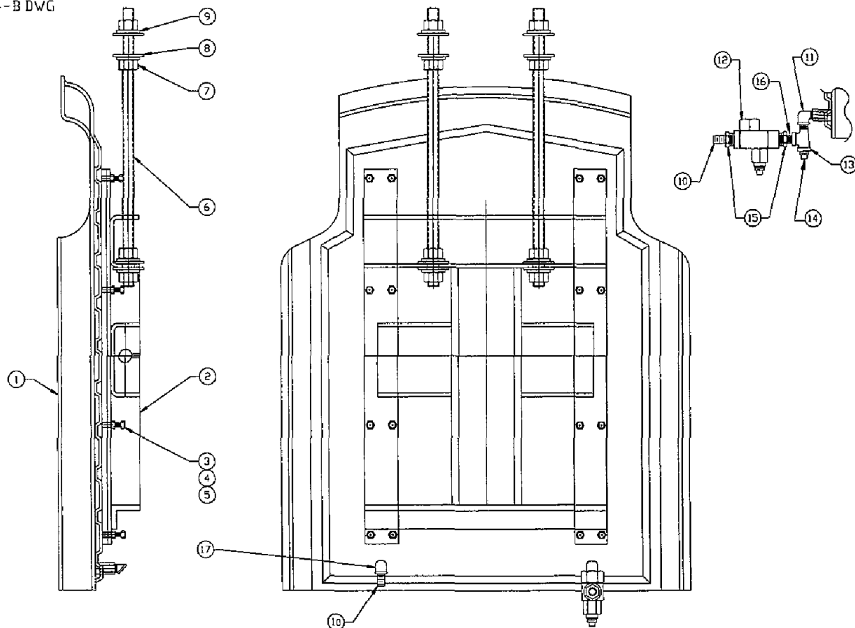
Figure 6-6. Rear Head Assembly
