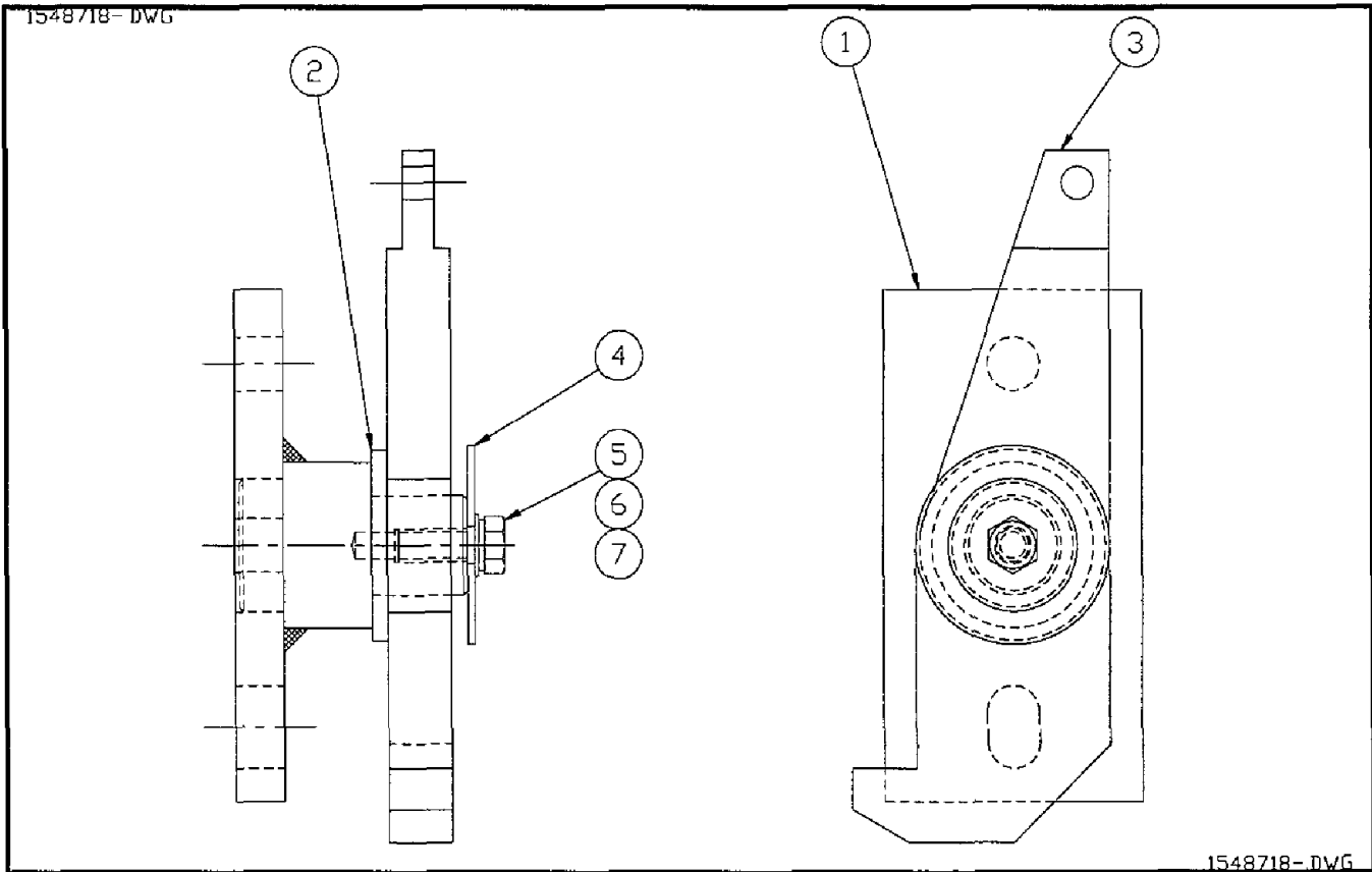
Figure 6-26. Locking Plate Assembly
