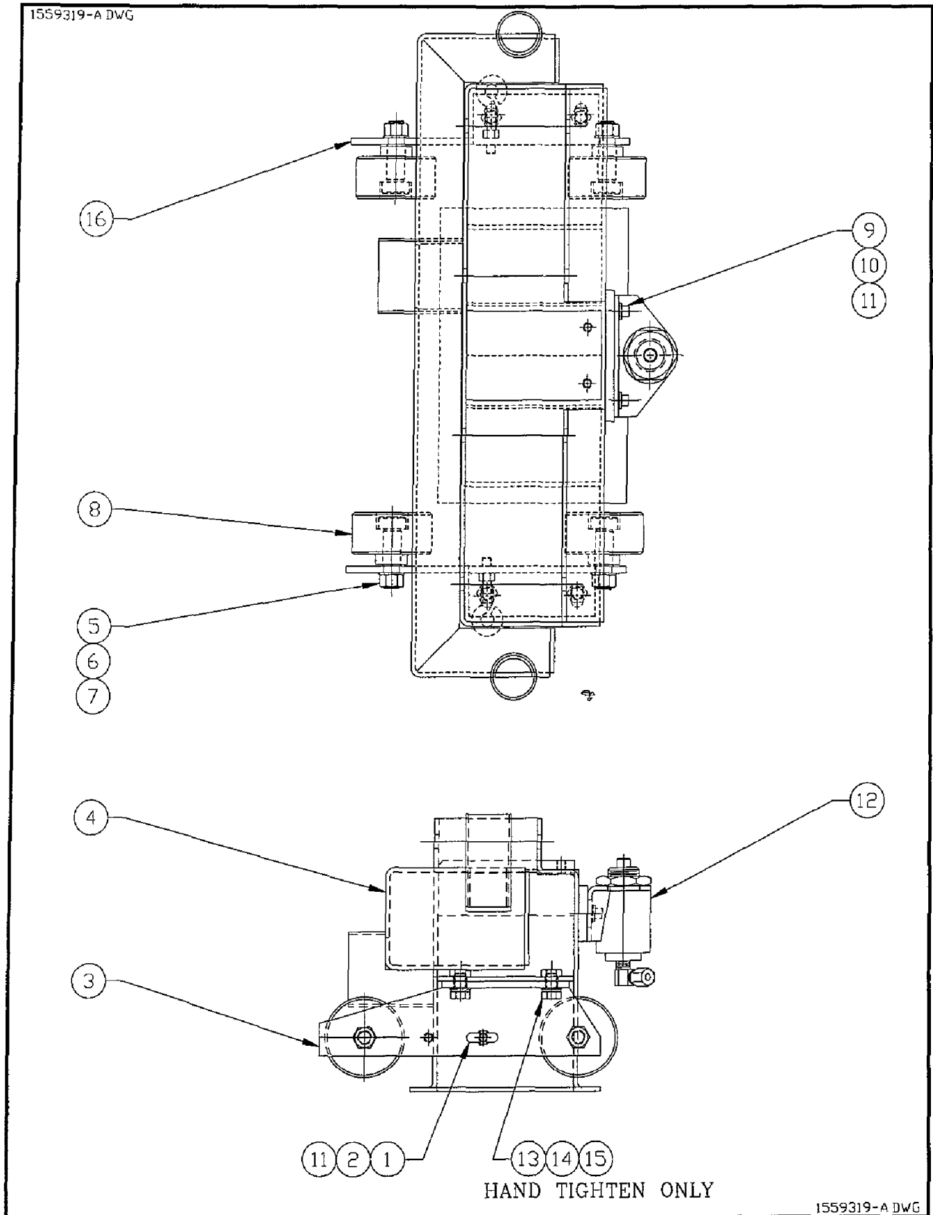
Figure 6-16. Receiving Tube Assembly
