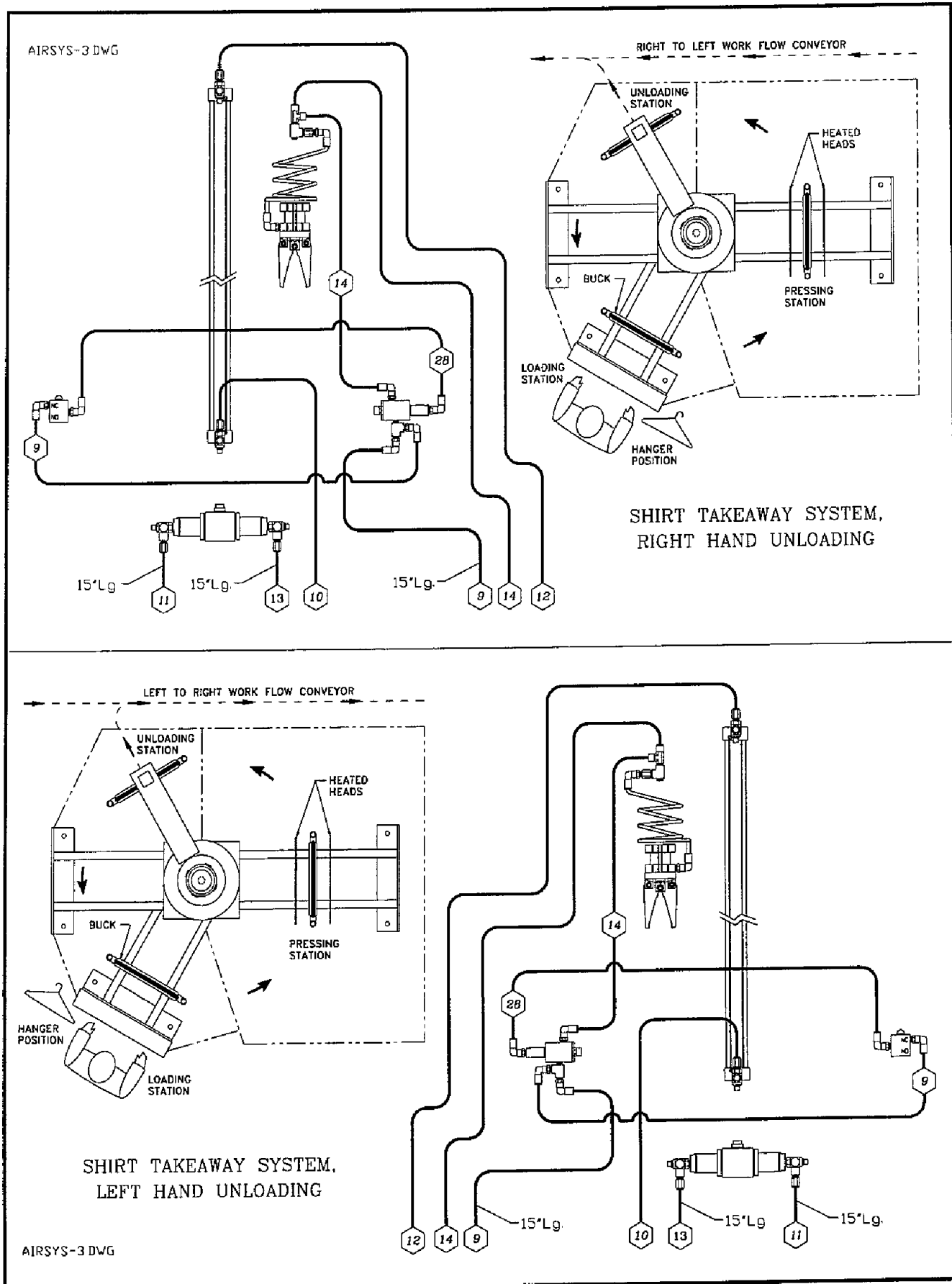
Figure 6-29. Air System, Triple-Pro (Sheet 3 of 3)
