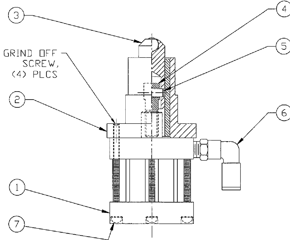
Figure 6-24. Detent Pin Assembly
