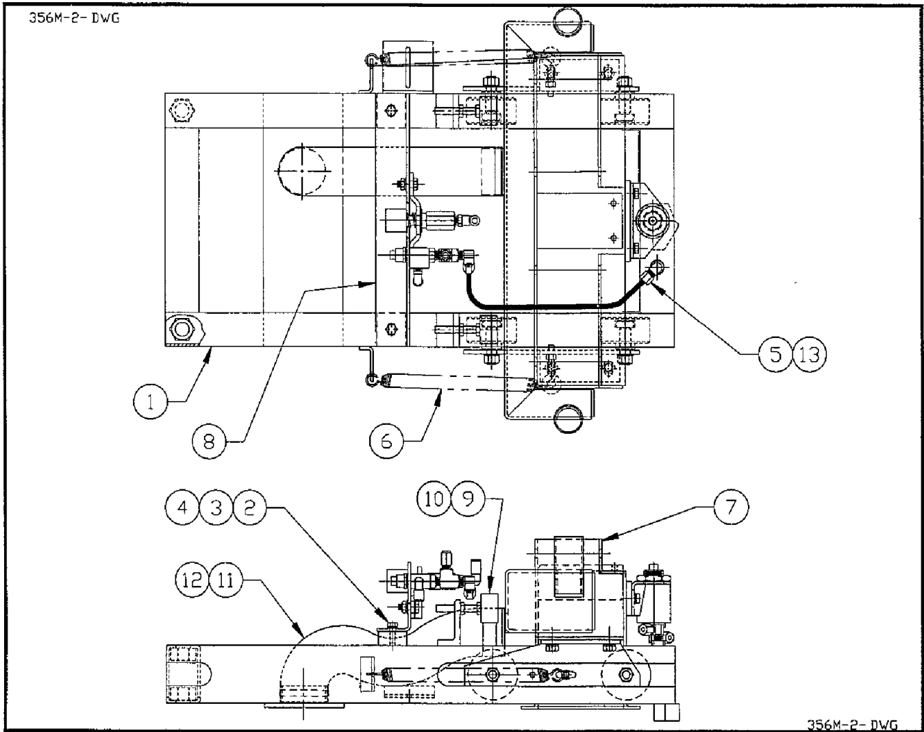
Figure 6-15. Buck Frame Sub-Assembly
