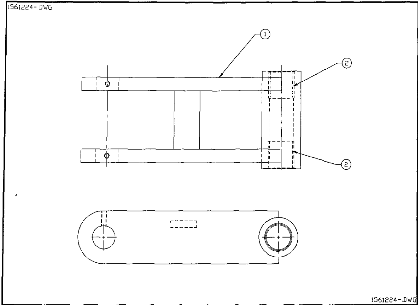
Figure 6-9. Lever Arm Assembly, Head Mounted
