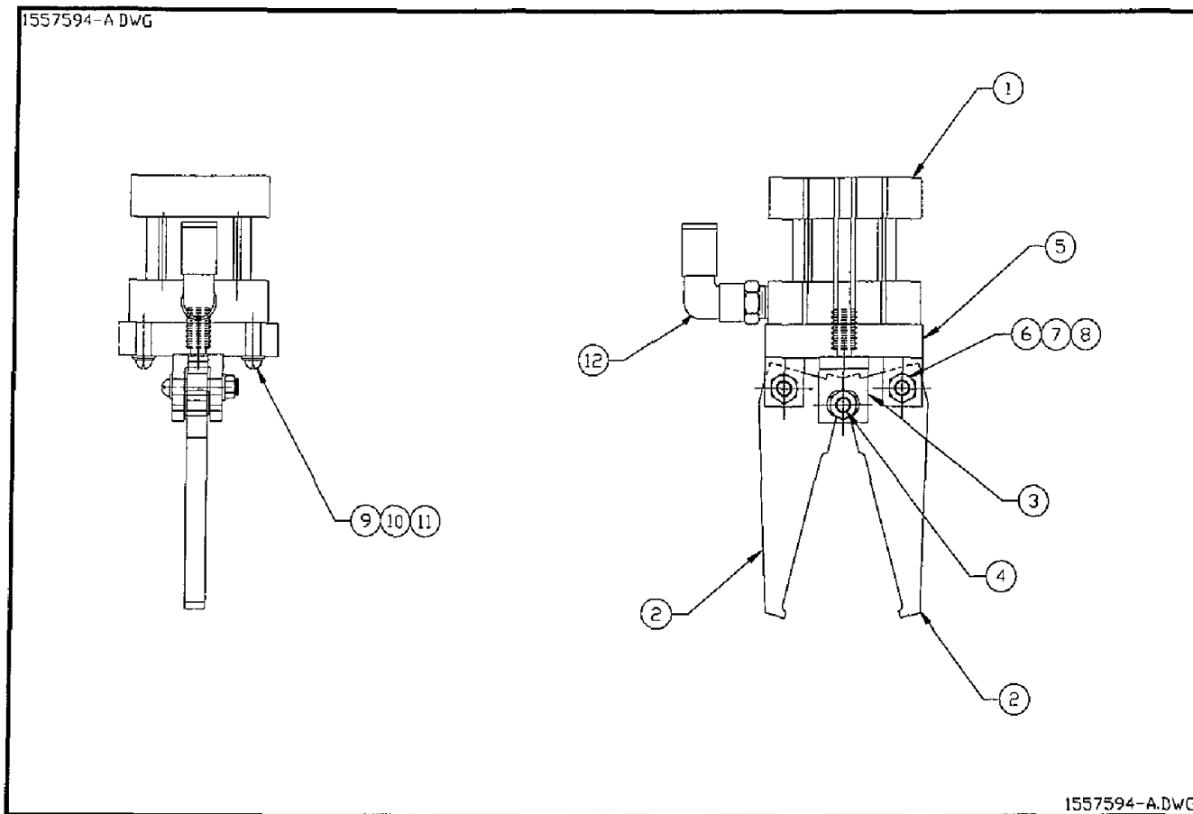
Figure 6-48. Gripper Assembly
