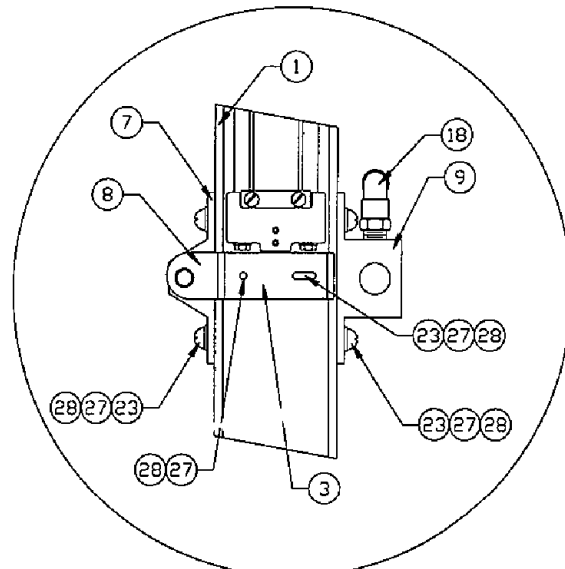
Figure 6-44. Shirt Take-Away, Right Hand Assembly (Sheet 2 of 2)
