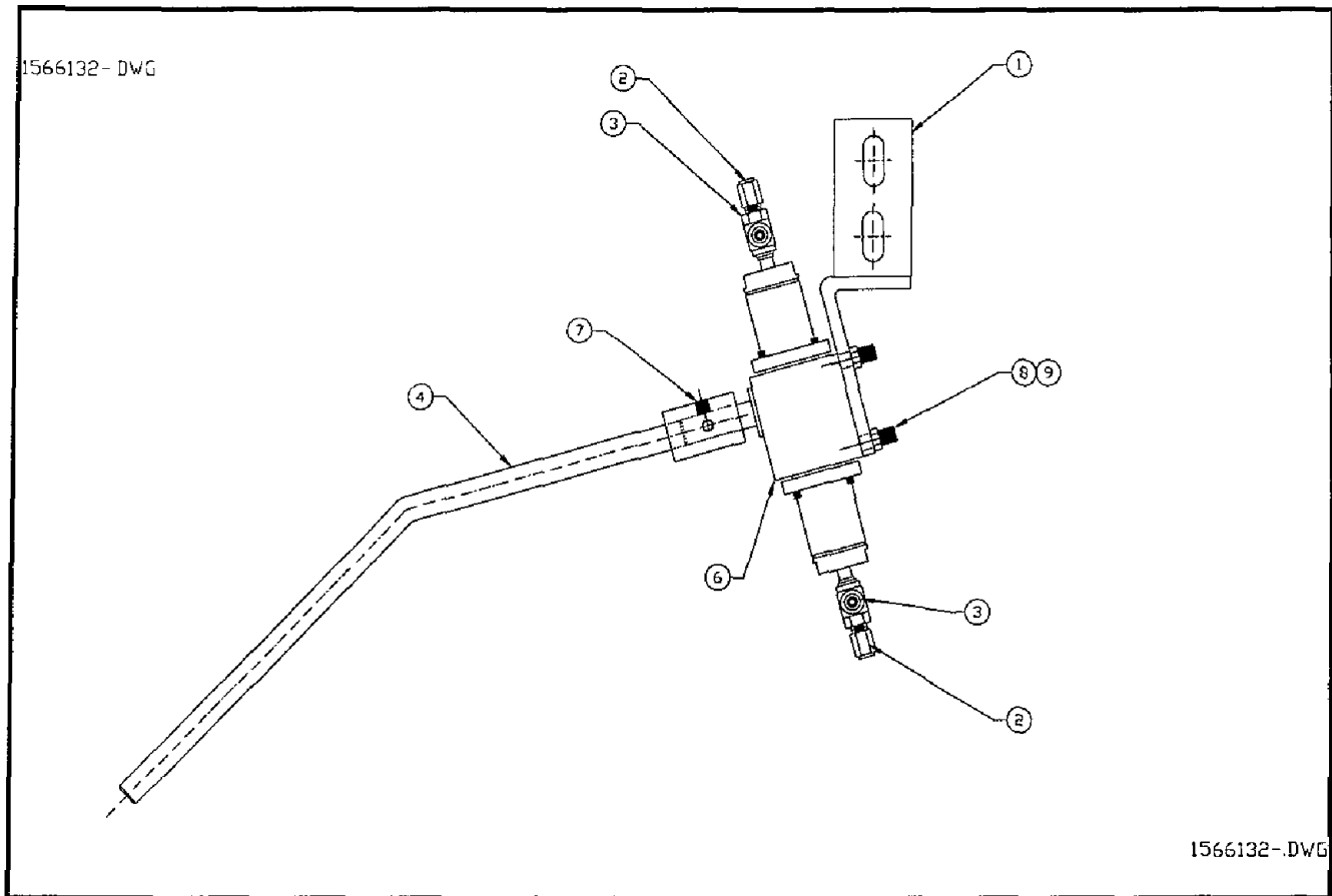
Figure 6-46. Mendline Assembly Option, Fits Right Hand Unloading
