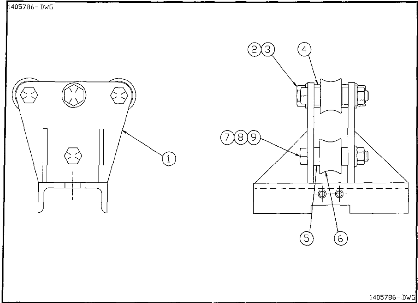
Figure 6-11. Roller Bracket Assembly
