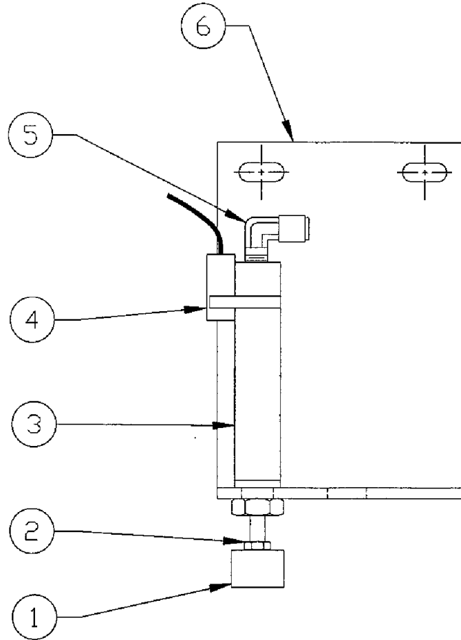
Figure 6-20. Air Cylinder and Bracket Unloading Station
