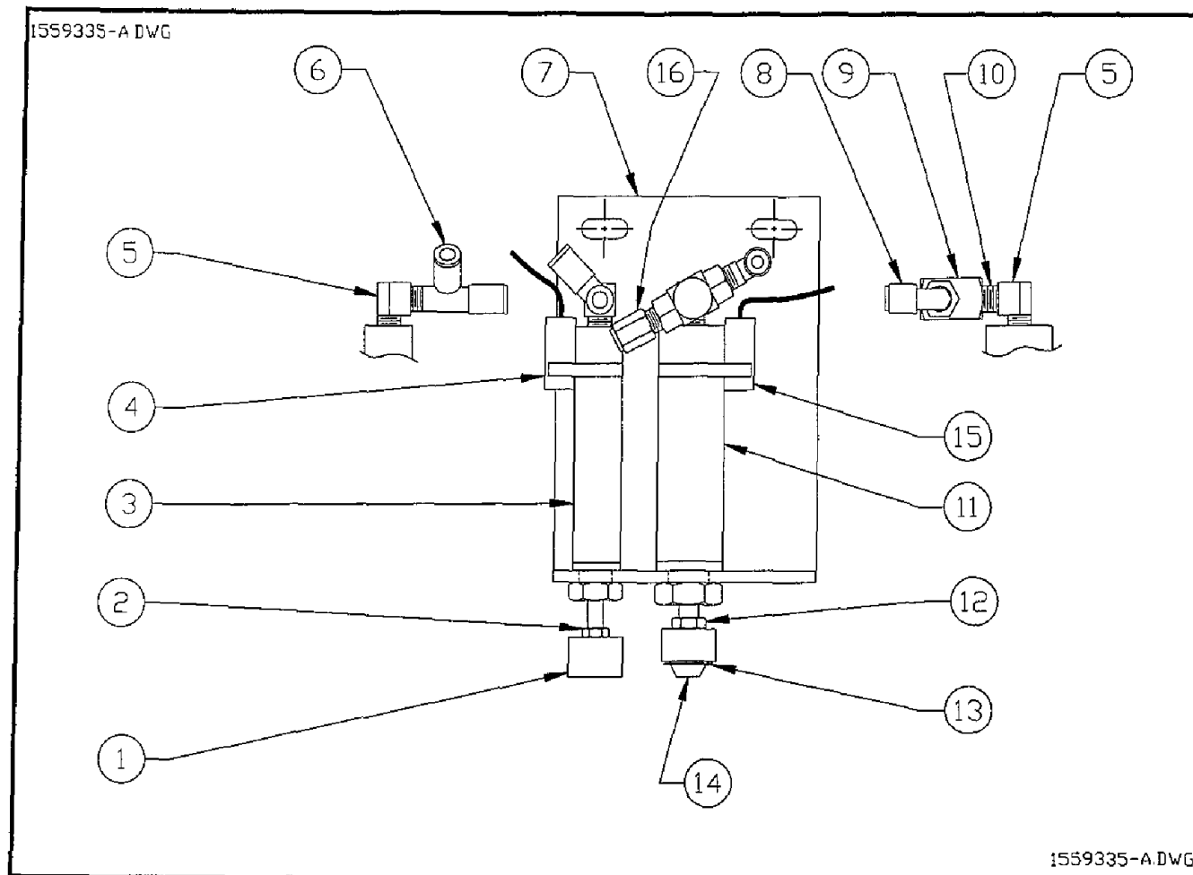
Figure 6-21. Air Cylinder and Bracket Dressing Station
