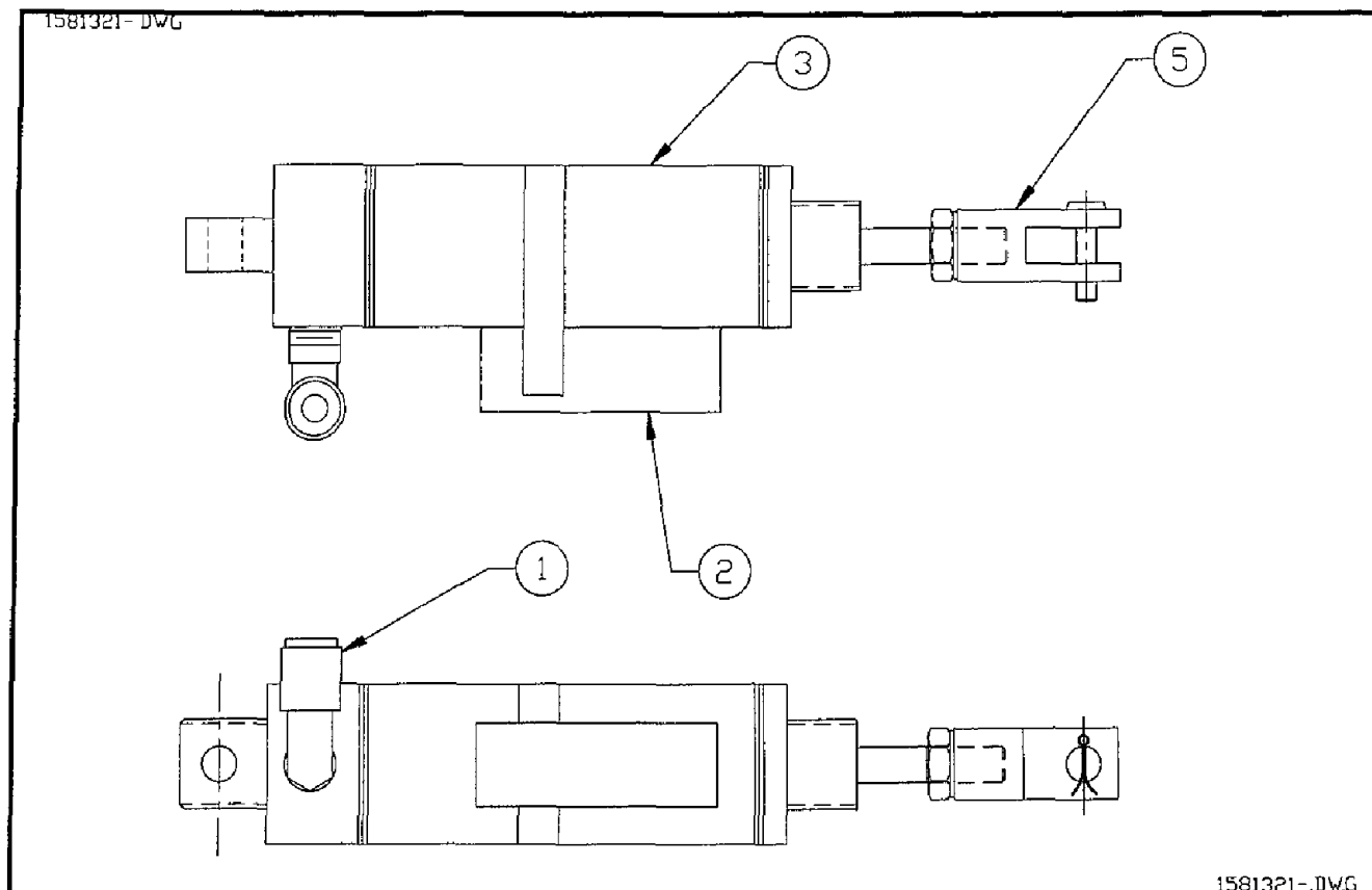
Figure 6-27. Locking Plate Cylinder Assembly
