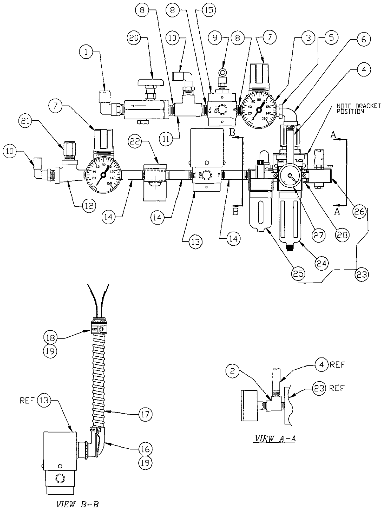
Figure 6-31. Air Inlet Assembly
