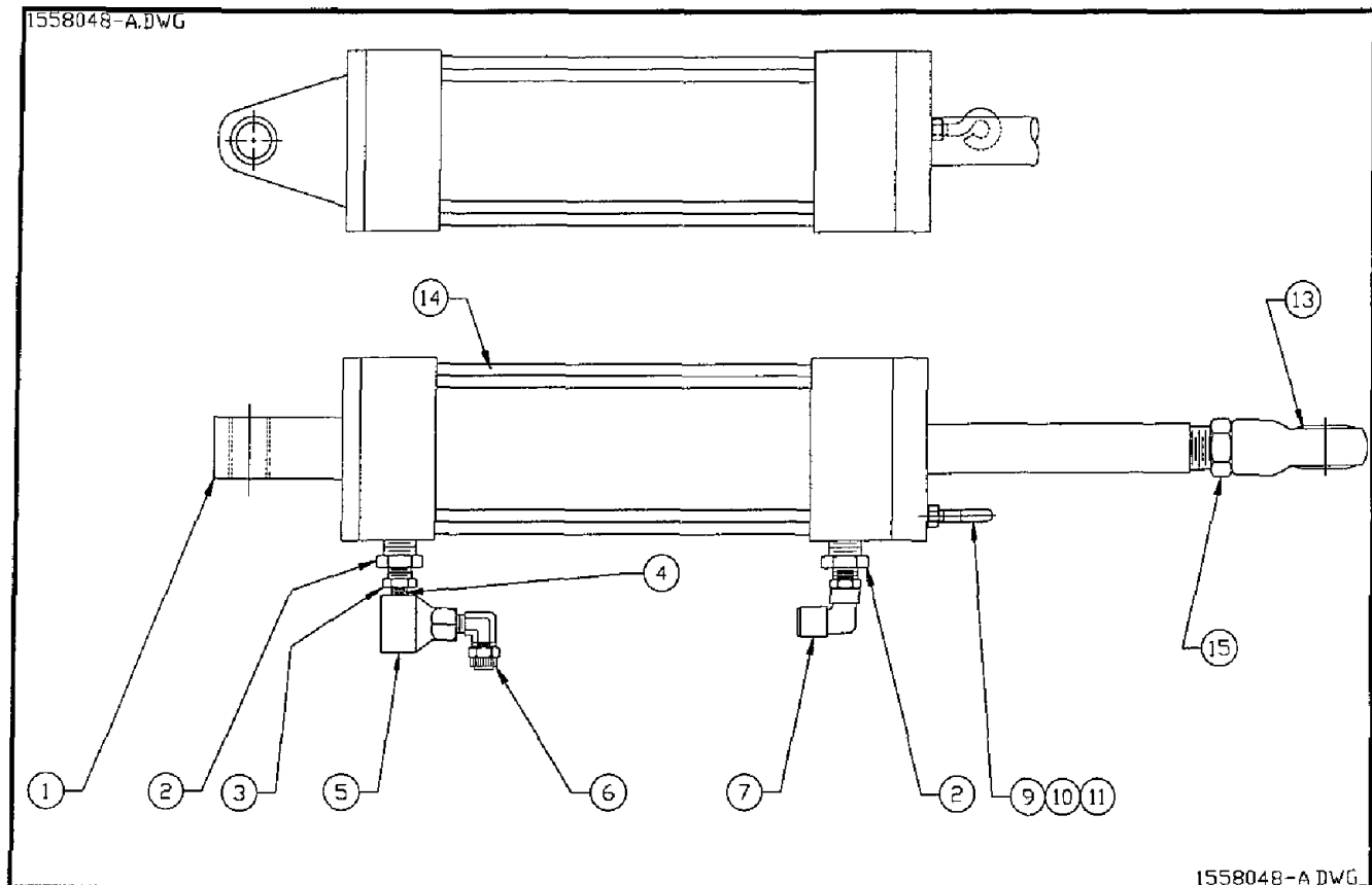
Figure 6-23. Air Cylinder Assembly, Indexing
