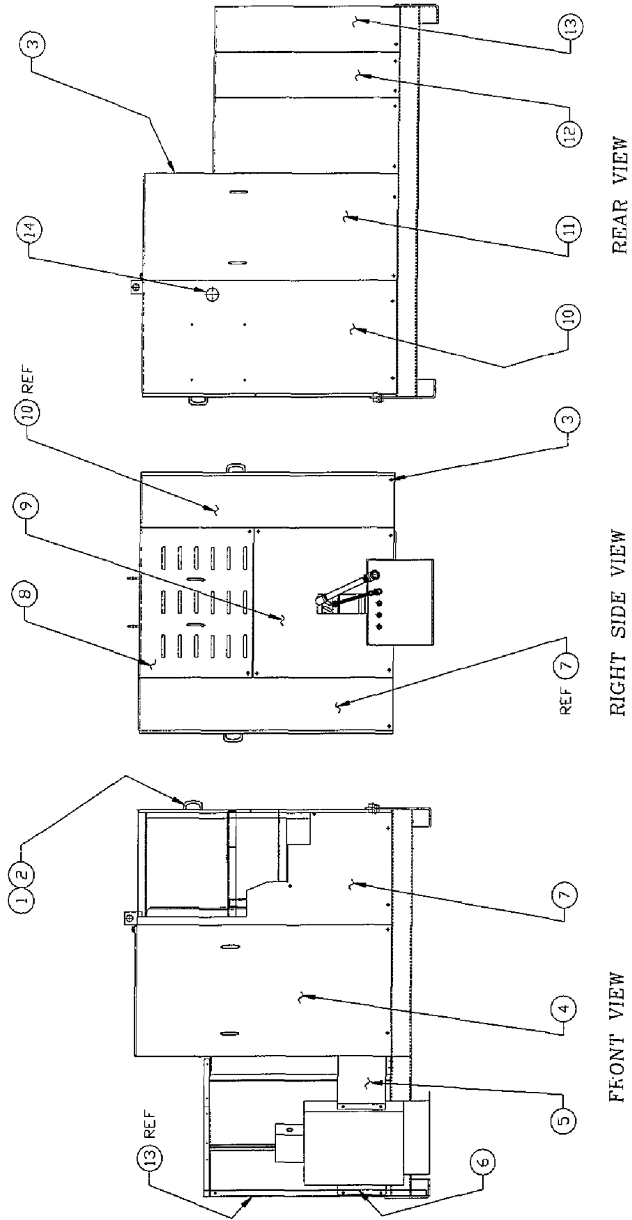
Figure 6-49. Covers
