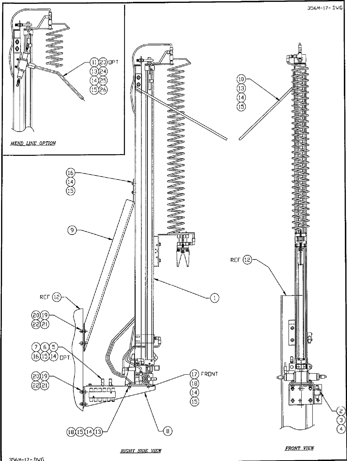
Figure 6-43. Shirt Take-Away System, Left Hand Unloading
