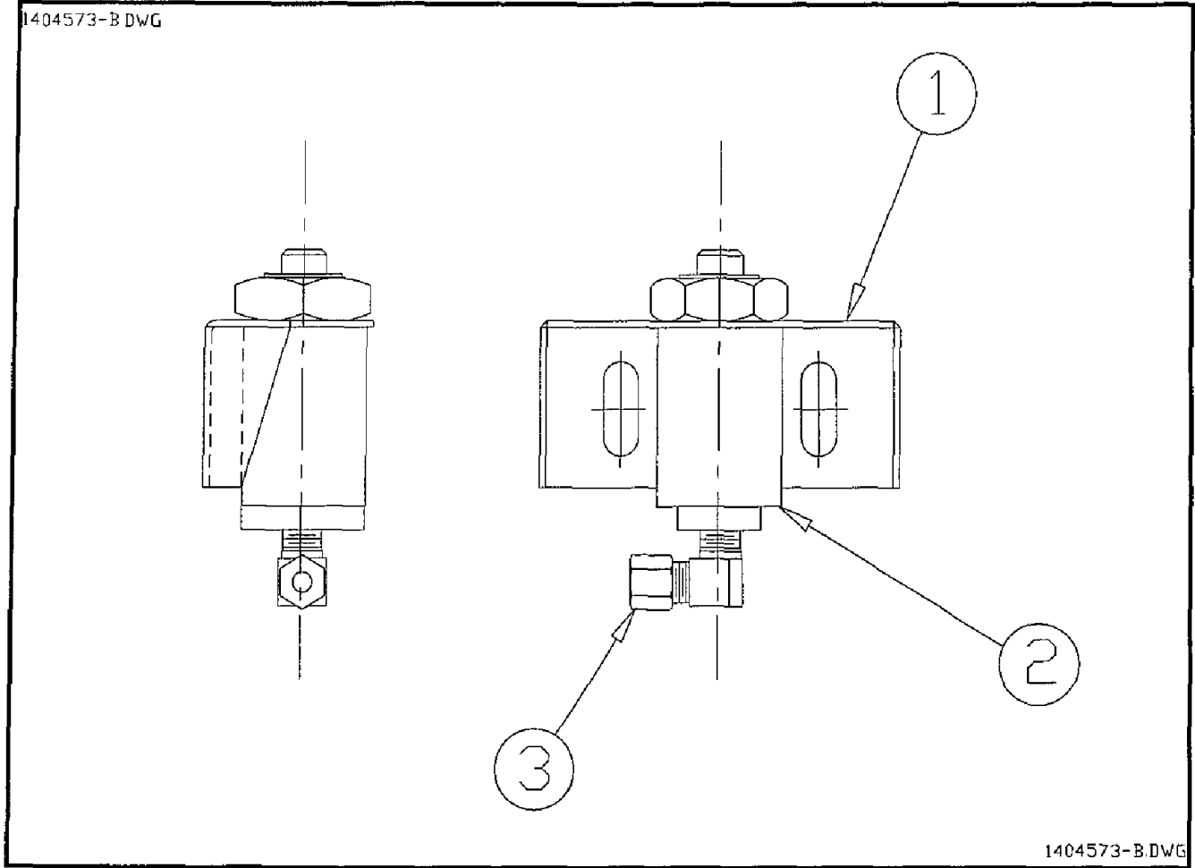
Figure 6-17. Tail Clamp Cylinder Assembly
